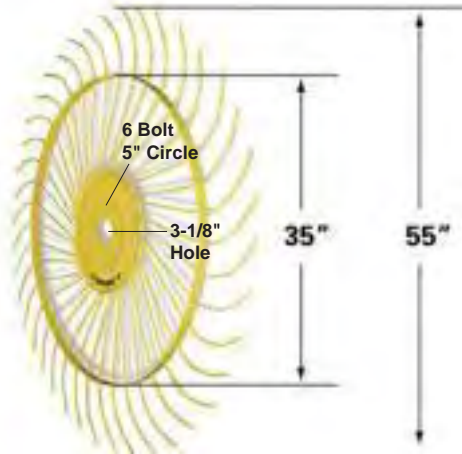
Left Hand Side (Uses 127-211 Tine) ORDER # P20BG002 $ 129.95
